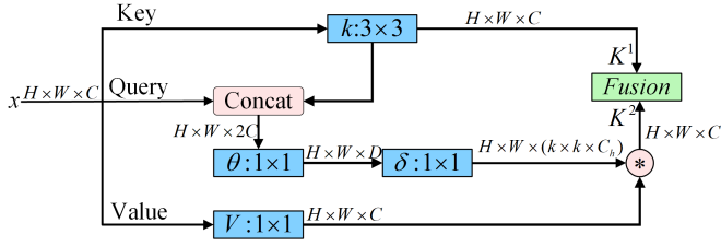
Fig. 4. Calculation details of CoT. denotes the matrix multiplication.
