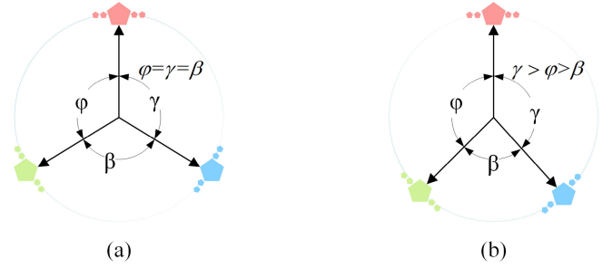
Fig. 5. Regular simplex. (a) Indicates that upon completion of the model training, all classes collapse to the vertices of a regular simplex, presenting a symmetrical configuration with equal angles. (b) Asymmetrical configuration with unequal angles.
