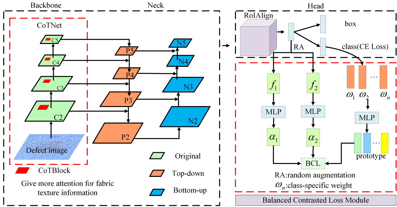
Fig. 2. Overall framework of the JDCBL consists of three main parts: backbone, neck, and head. The framework deploys CoTNet as the backbone to enhance local feature representation, generating multiscale feature maps (C2–C5). These feature maps are fed into PAFPN, which adaptively focuses on defect-related features across different scales. The head module then performs defect localization and classification using the fused features. Additionally, BCL is integrated into the training process to address class imbalance and reduce bias toward tail classes.
