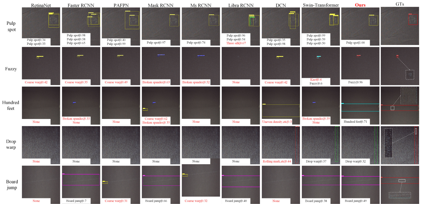
Fig. 7. Comparison of detection effects of several methods on tail classes.
