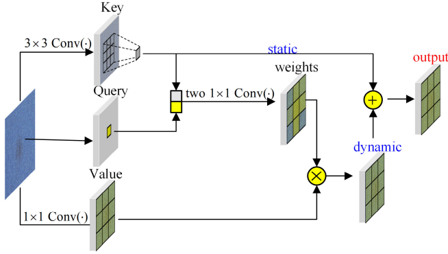
Fig. 3. Structure of CoT. The key and value of the input image are obtained through 3 \times 3 convolution and 1 \times 1 convolution, respectively, and then the key is concatenated with the query and the context weight of the image is obtained through two 1 \times 1 convolutions. The dynamic information is multiplied by the value and fused with the key representing the static information to get the final output.
